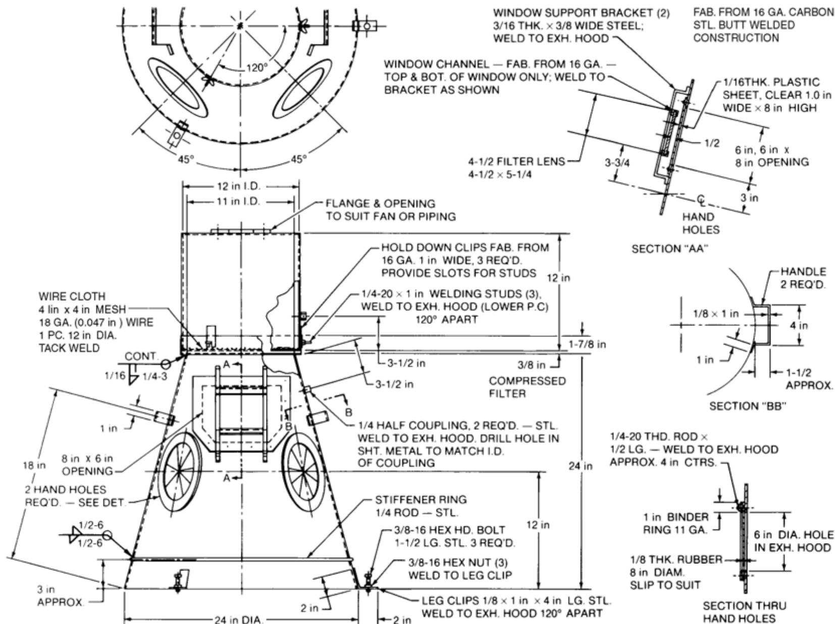
Figure 1 – Suggested Test Chamber
