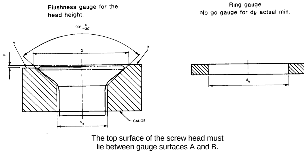
Figure C2. Gauging method
