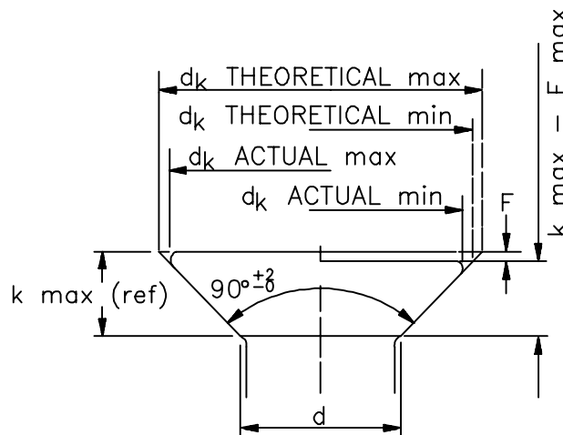
Figure C1. Head configuration
