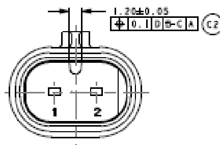
Figure 11: GM Mating Connector on Sensor Harness, Figure B1 with Circuit Identification
