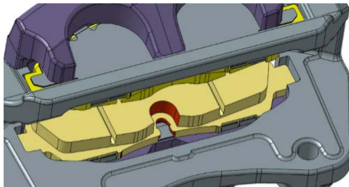
Figure 10: Backing Plate/Brake Pad Accommodation
