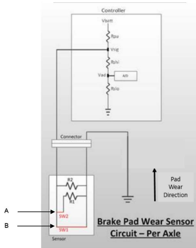
Figure 1: Electrical Circuit Diagram, Diagnostics
