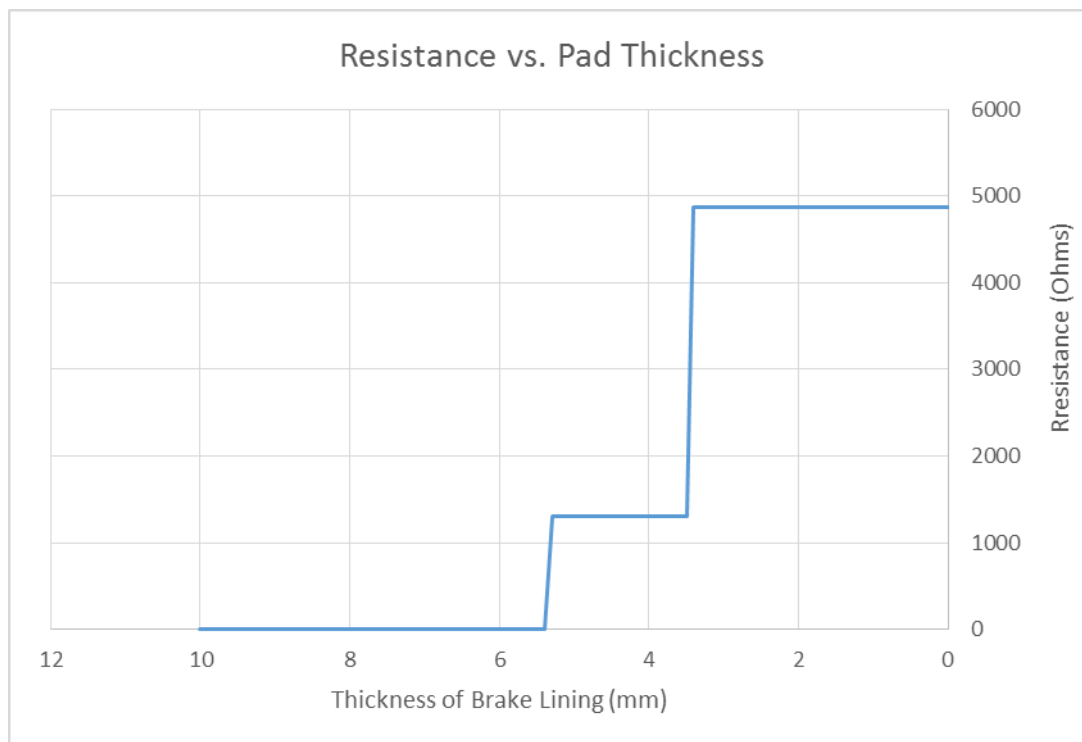
Figure 4: Typical BPWS Output (Example)
