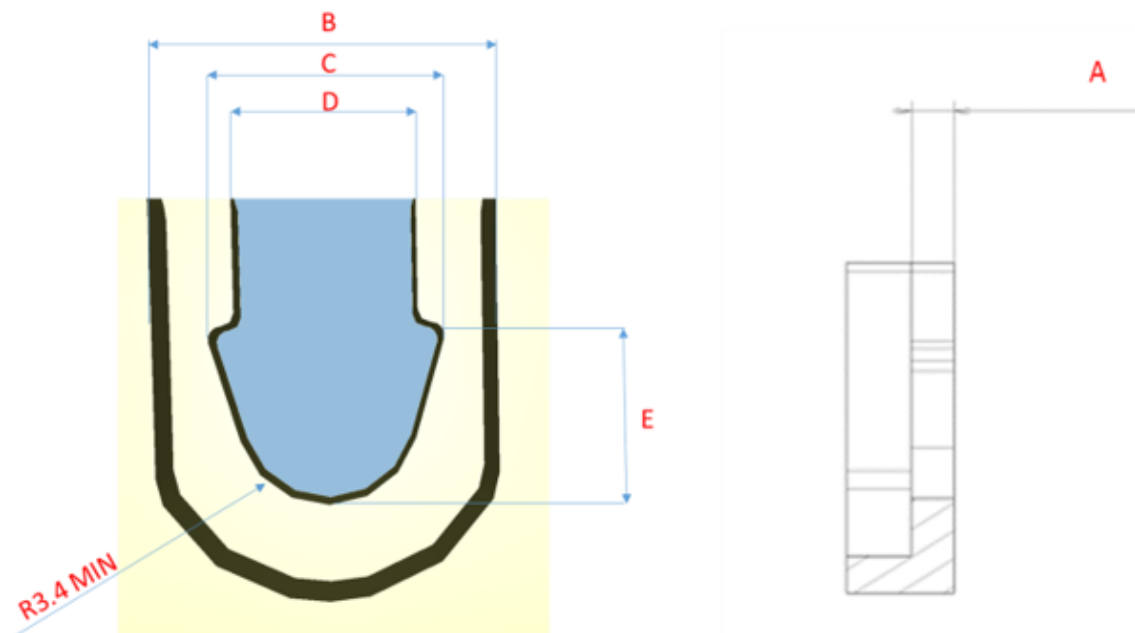
Figure 9: Pad/Backing Plate Cutout Geometry
