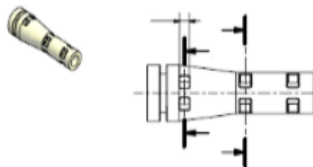
Figure 6: Sample Trumpet Grommet Geometry
