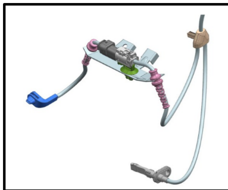
Figure 3: Recommended Sensor Interface
