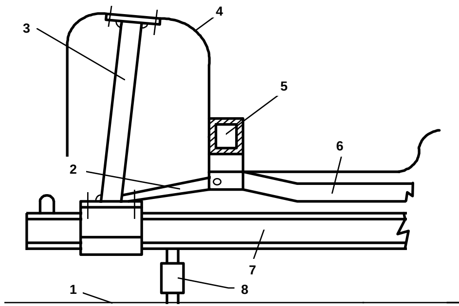
Fig. 1: Front bar fixation of body in white
