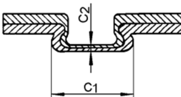
Figure 1: Clinch Weld Size Measurements
