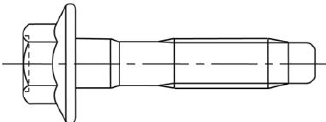
Figure 2: Metric Hexagon Bolt with Heavy Flange and M-Point (Reduced Body)
