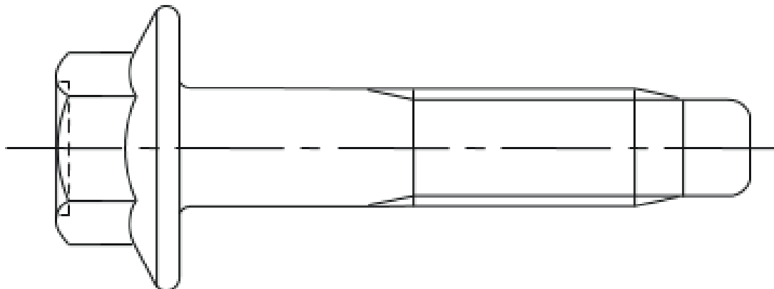
Figure 1: Metric Hexagon Bolt with Heavy Flange and M-Point (Full Body)
