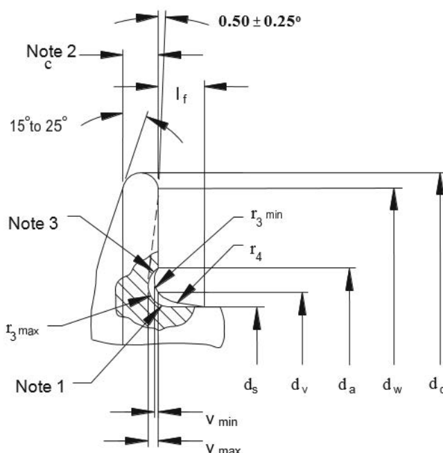
Figure 4: Dimensions of Metric Hexagon Bolts with Heavy Flange and M-Point for Long Bolts Type U Fillet
