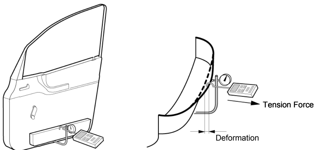
Figure 5: Measurement of Tensile Deformation of Primary Door Storage Compartment
