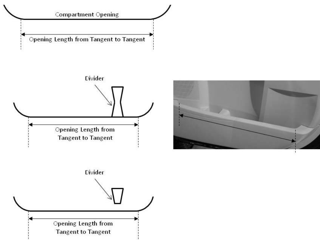
Figure 2: Measurement of Opening Length for Tensile Testing
