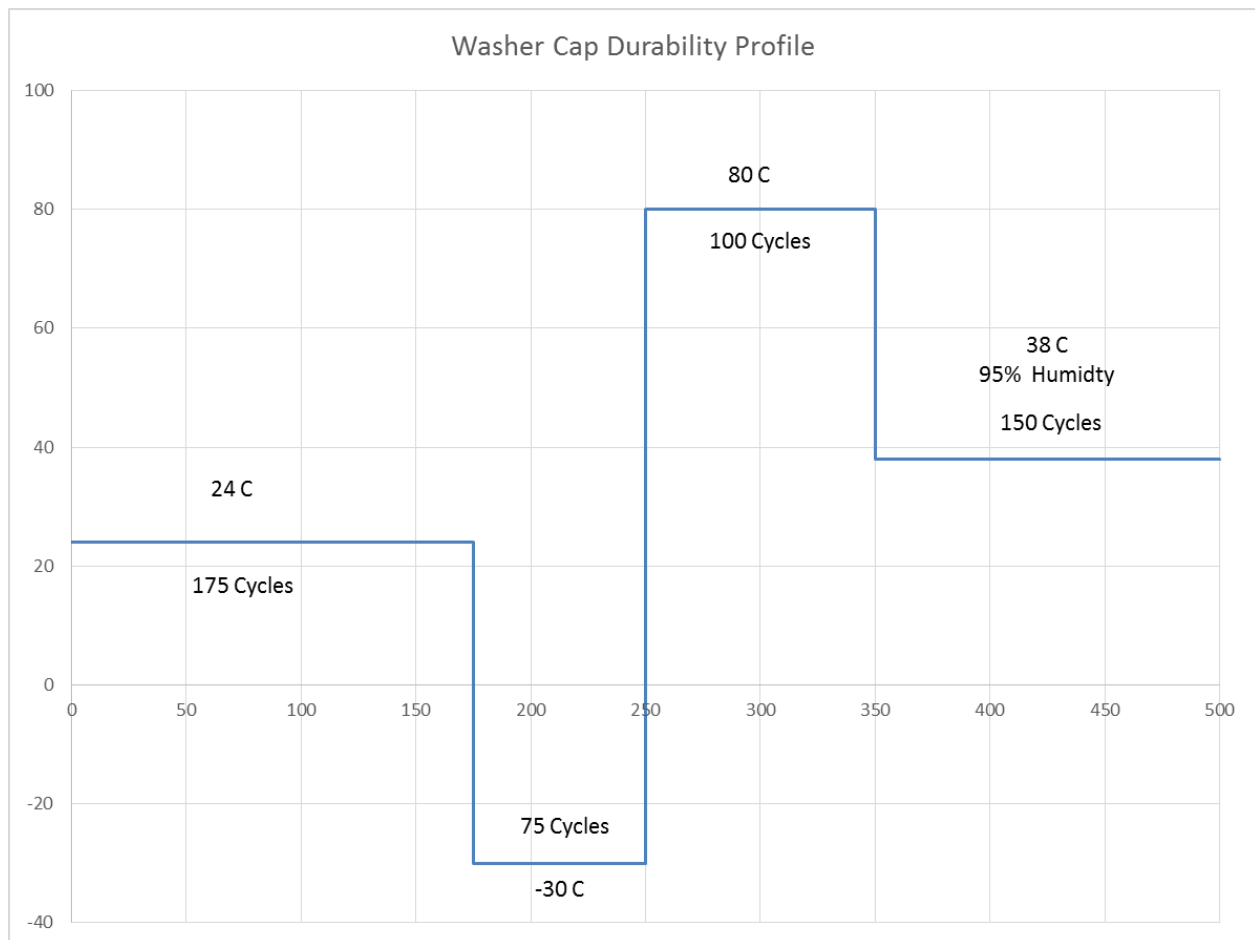
Figure 2: Durability Profile for Passenger Vehicles
