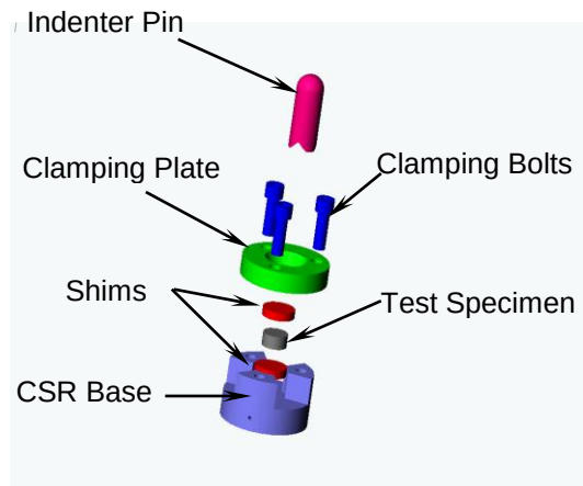
Figure 1: CSR Fixture Components
