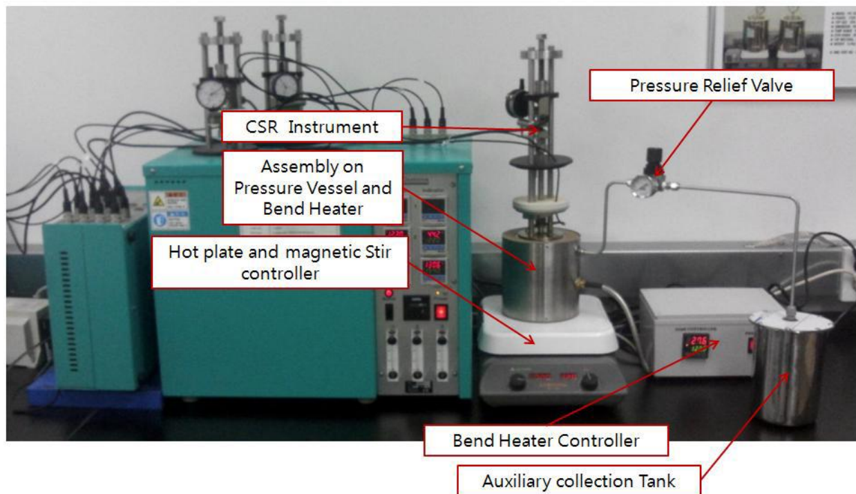
Figure 4: GMW16678 Test Setup (Courtesy of Dong-Ah Manufacturing Company)
