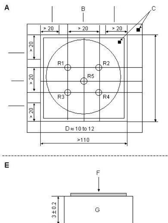
Figure 1: Base with Glass Plate Placed on Spacer and Reference Marks for Positions and Centering of the Reflectometer for Determination of Reflectance Values
