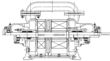
Figure 5 TWO STAGE, FLAT PORT PLATES
