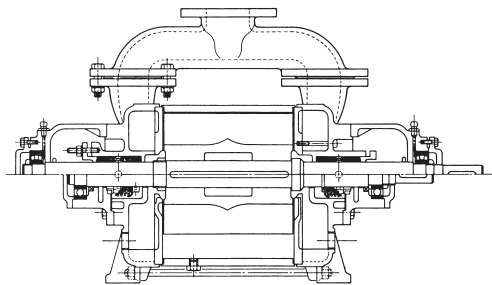
Figure 3 SINGLE STAGE, FLAT PORT PLATES
