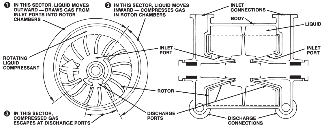
Figure 2 CONICAL PORT
