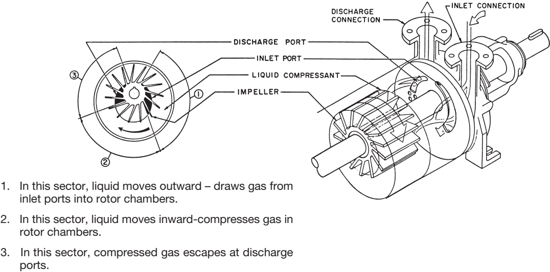
Figure 1 FLAT PORT PLATE
