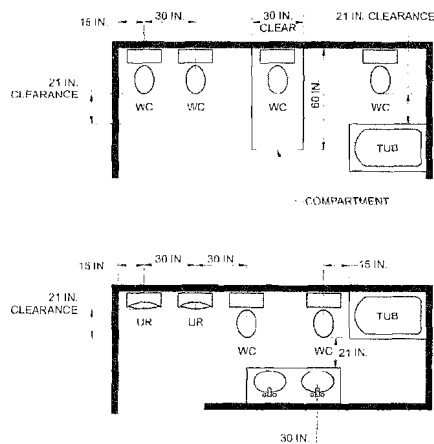
FIGURE 405.3.1 FIXTURE CLEARANCE
