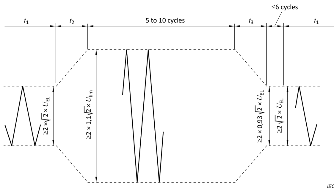
Figure 3 – Time and amplitude limits for an overvoltage period waveform
