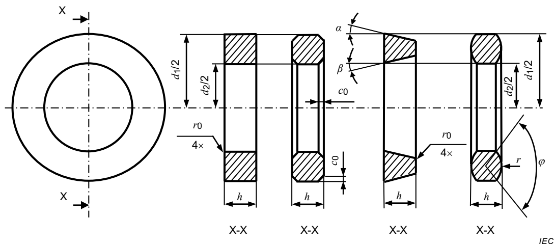
Figure 1 – Ring cores
