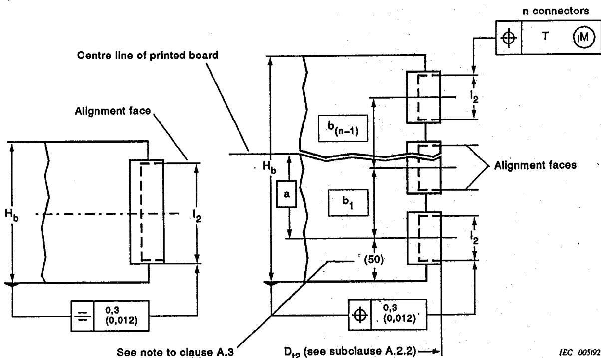
Figure 12 - Position of connectors on plug-in units for subracks greater than 3U
