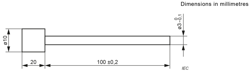
Figure 101 – Test rod for interlock concealment
