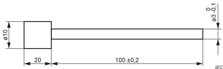
Figure 101 – Test rod for interlock concealment
