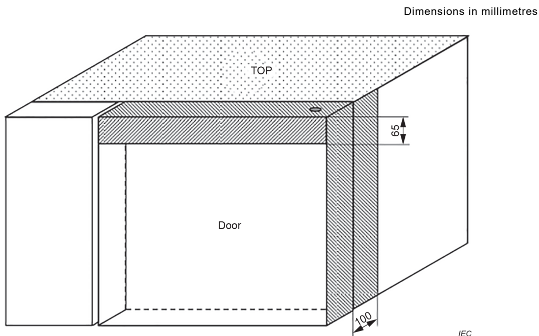
Figure 105 102 – Adjacent surfaces which are not measured
