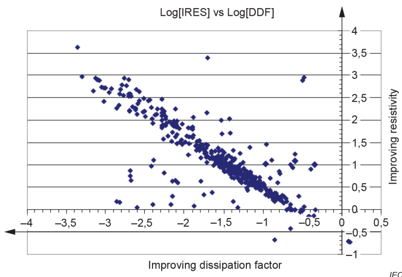
Figure 3 – Correlation between resistivity and dissipation factor [6]
