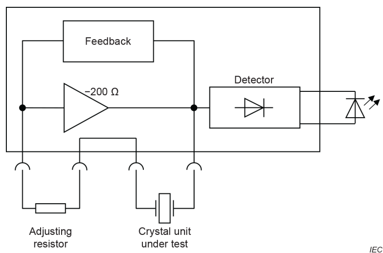
Figure B.4 – Block diagram of circuit system
