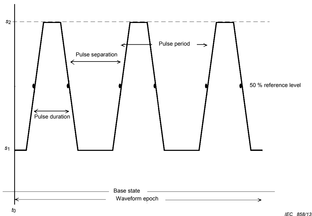
Figure 7 – Pulse train
