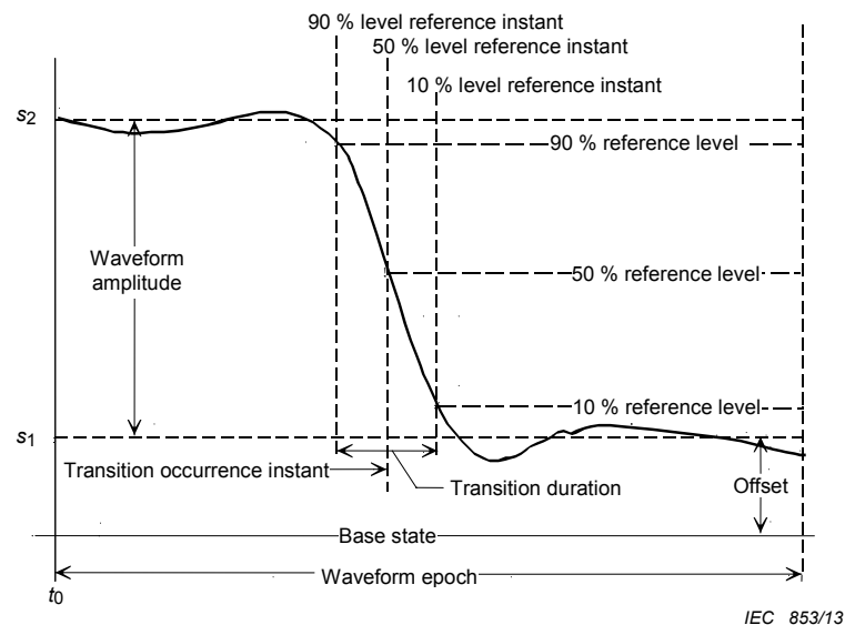
Figure 2 – Single negative-going transition
