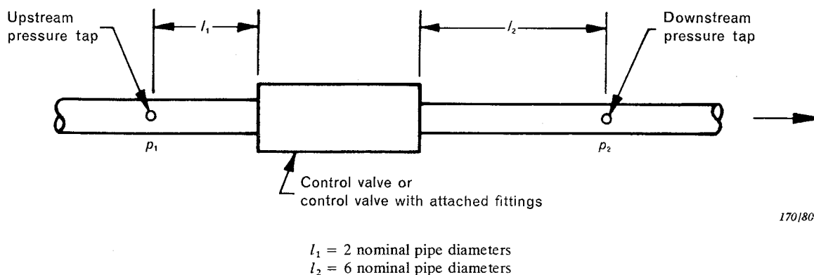
FIG. 1. — Pressure tap locations
