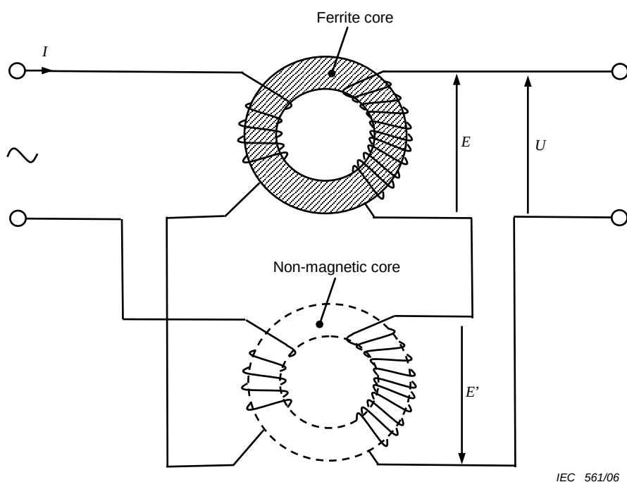
Figure 7 – Test sample with compensation unit
