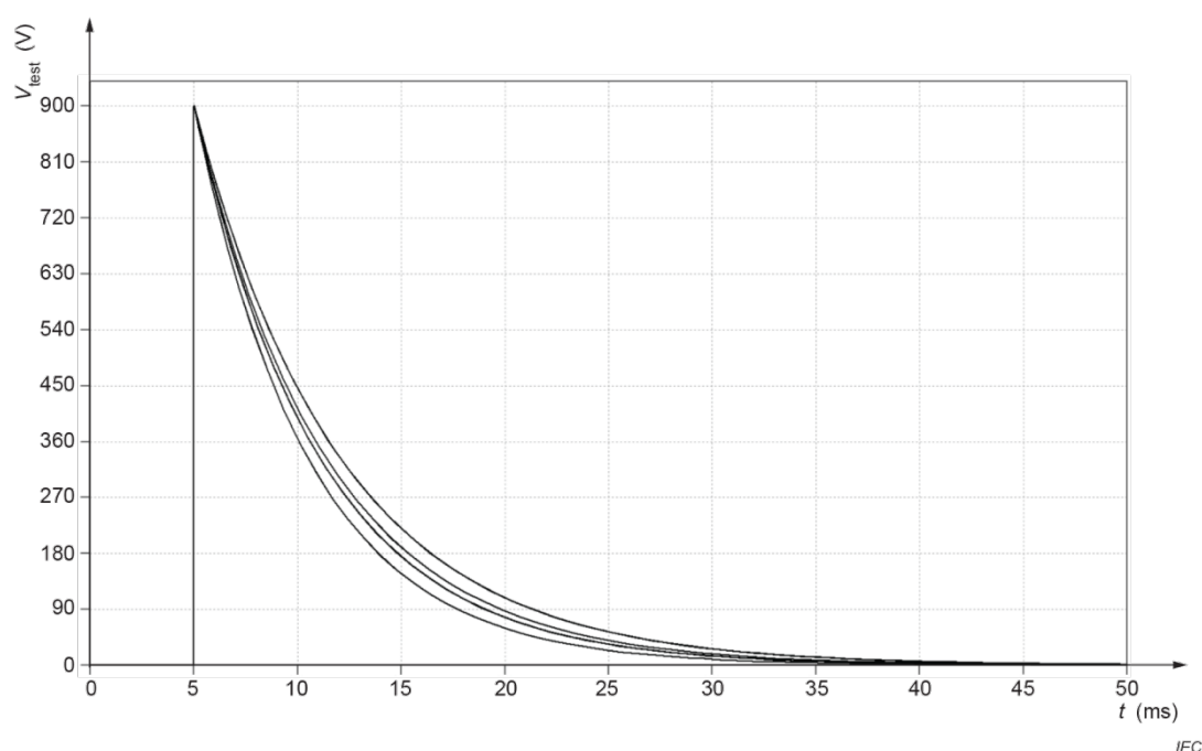
Figure AA.4 – Defibrillation PULSE generated by the defibrillation test generator from Figure AA.3
