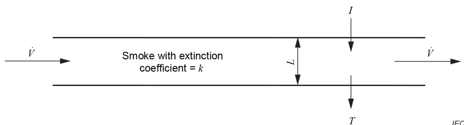
Figure 4 – Dynamic smoke measurement
