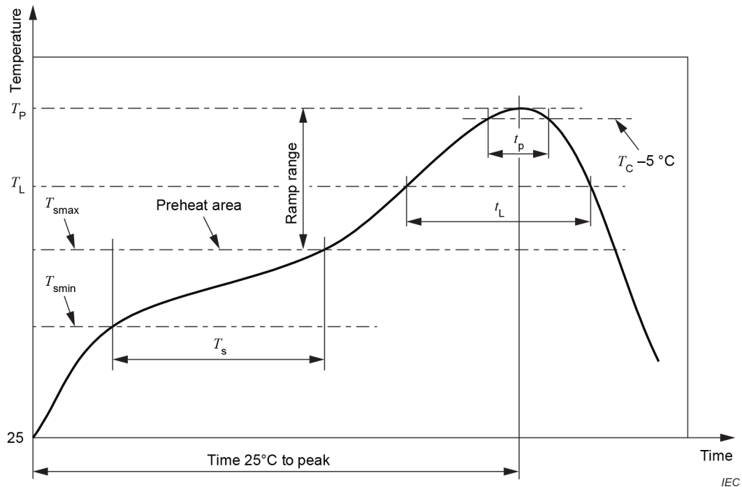
Figure A.11 – Classification profile
