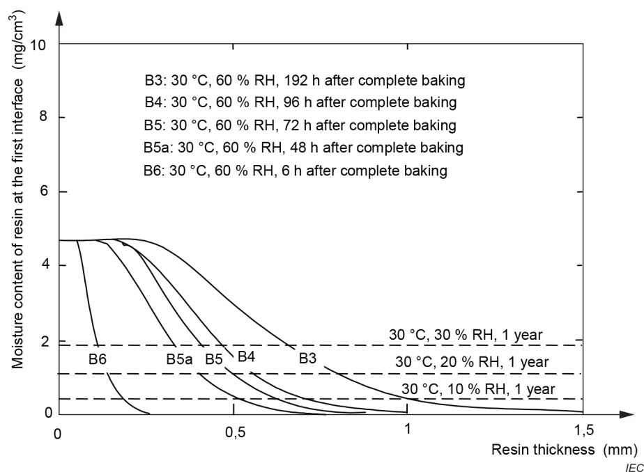
Figure A.7 – Dependence of the moisture content of resin at the first interface on resin thickness related to method B of moisture soak
