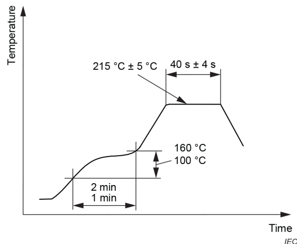
Figure A.12 – Temperature profile of vapour-phase soldering (condition B-A)
