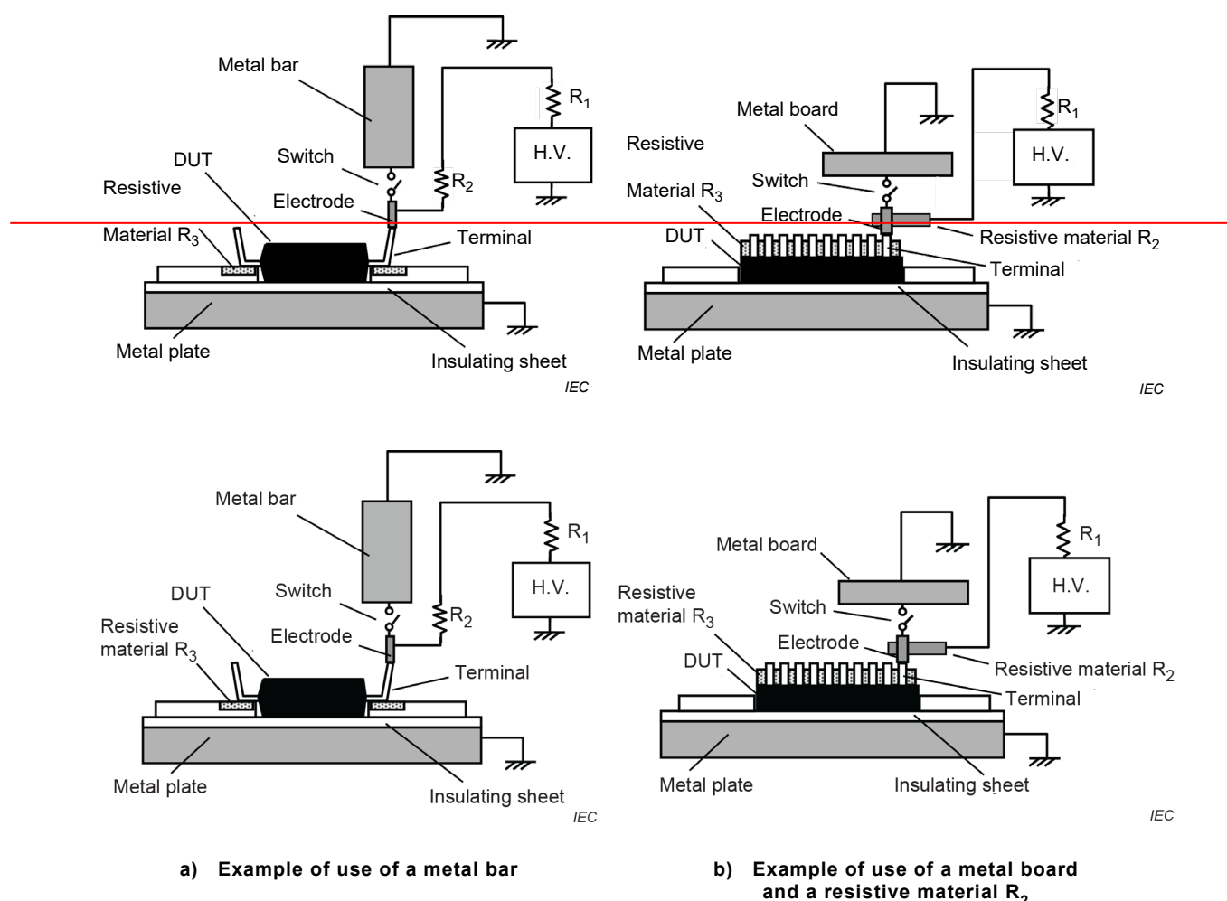
Figure J.1 – Examples of discharge circuit where the discharge is caused by closing the switch
