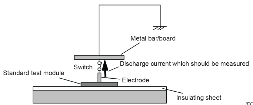
Figure J.2 – Verification test equipment for measuring the discharge current flowing to the metal bar/board from the standard test module
