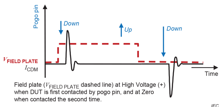
Figure G.2 – Dual discharge procedure (field charging, 1 st I_{\text{CDM}} pulse, no field, 2 nd I_{\text{CDM}} pulse)
