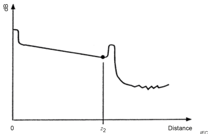
Figure B.4 – Schematic trace of a specimen sample (0 to z_2 ) with no section preceding it (single-point technique 0 (B.4.3.2))
