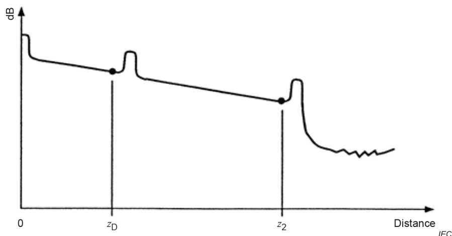
Figure B.4 – Schematic trace of a specimen sample (0 to z_2 ) with no section preceding it (single-point technique 0 (B.4.3.2))
