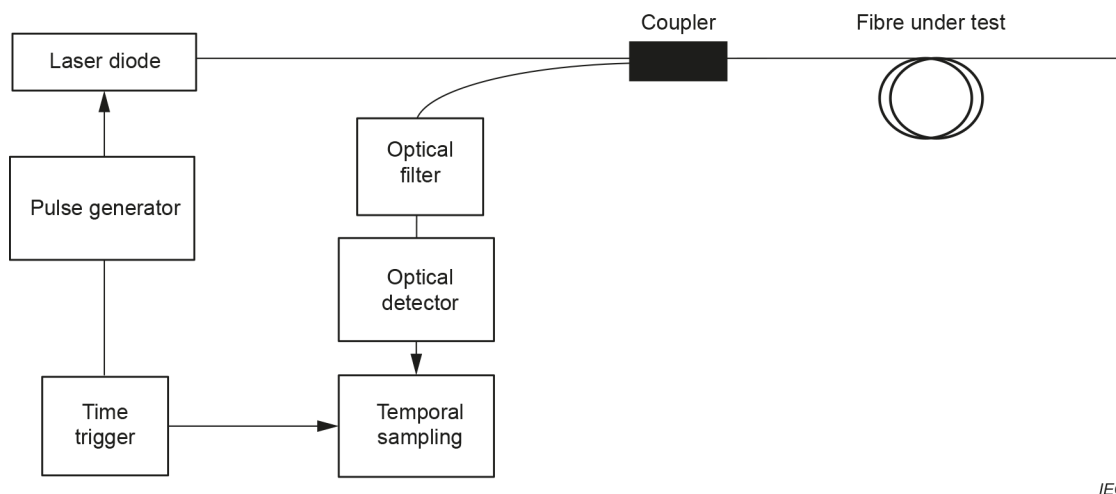
Figure F.1 – Equipment setup for BOTDR technique
