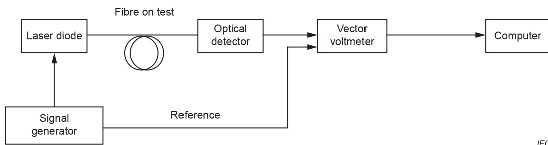
Figure C.1 – Equipment set-up for phase-shift technique (C.2.2.2)
