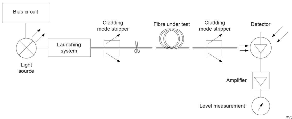
Figure A.1 – Arrangement of equipment to make for loss measurement at one a specified wavelength
