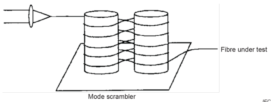
Figure A.8 – Mode scrambler (for A.4 fibre)
