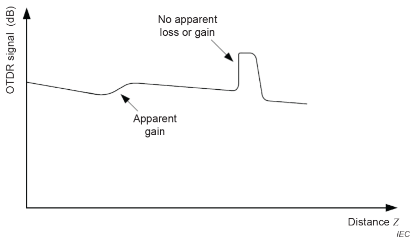
Figure C.5 – Schematic of an expanded OTDR trace showing two point discontinuities, one with apparent gain, and another with no apparent loss or gain
