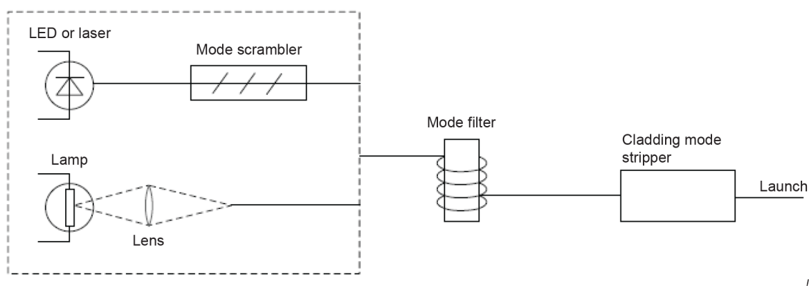
Figure A.3 – General launch arrangement
