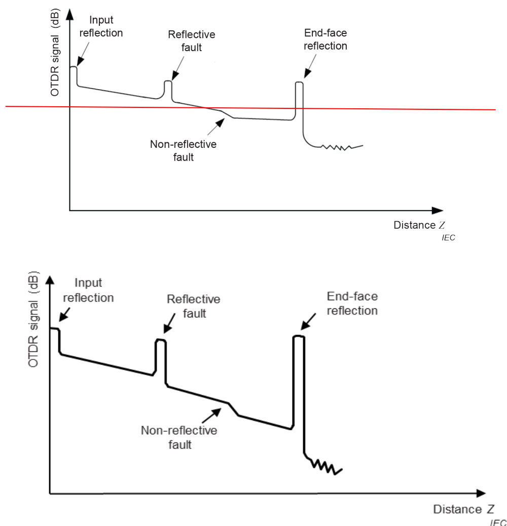
Figure C.4 – Schematic OTDR trace showing apparent loss due to point discontinuities, one reflective and one non-reflective
