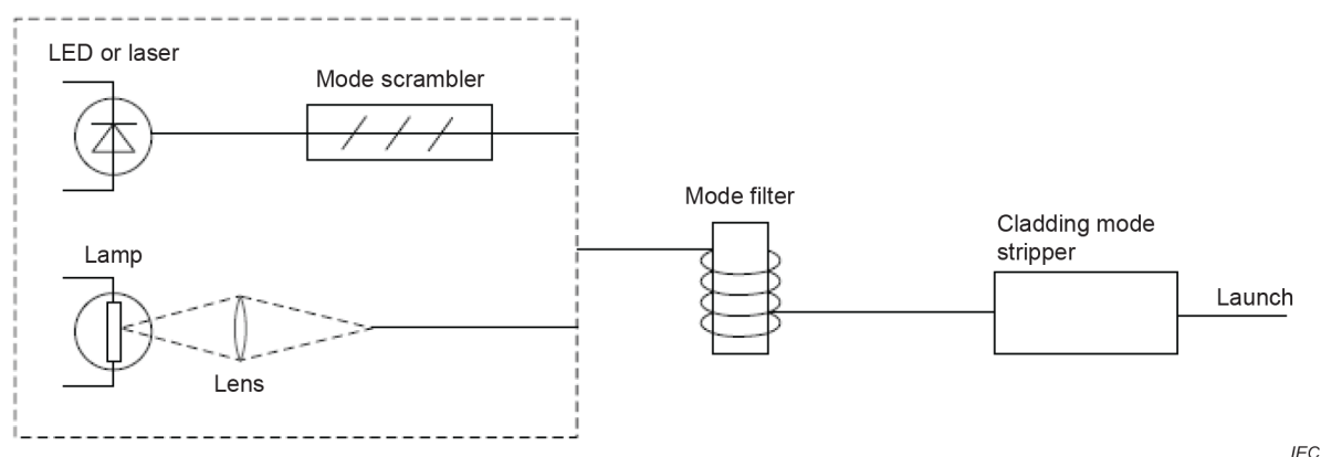
Figure A.3 – General launch arrangement
