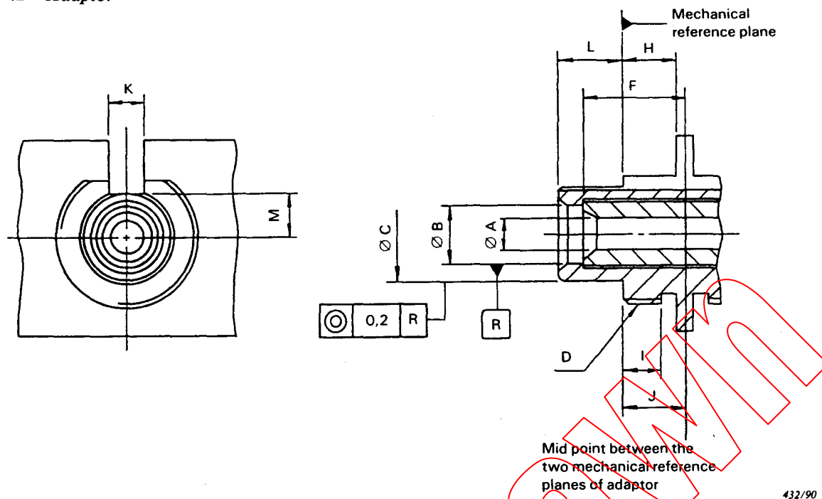
Figure 2 — Adaptor (dimensions given in Table 2)
