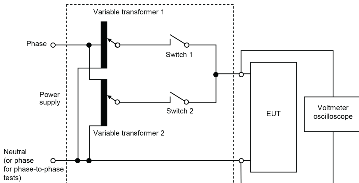
a) Schematic of test instrumentation for voltage dips, short interruptions and voltage variations using variable transformers and switches
