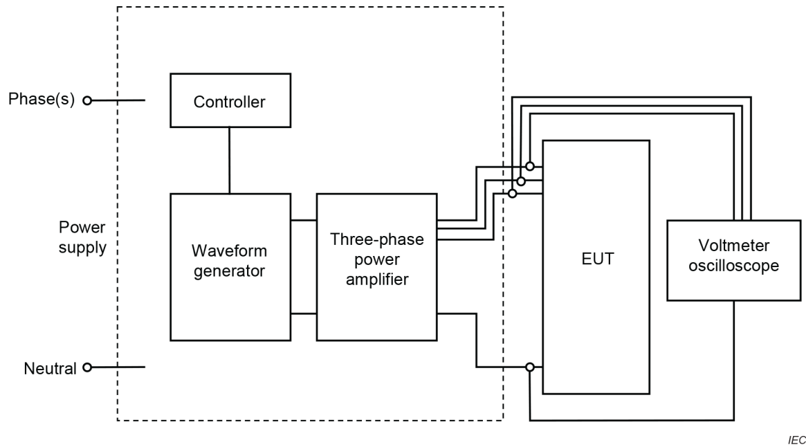
Figure C.2 – Schematic of test instrumentation for three-phase voltage dips, short interruptions and voltage variations using a power amplifier
