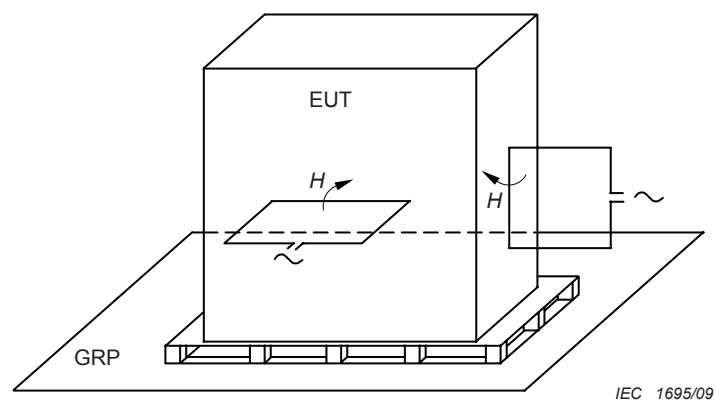
Figure 6 – Example of investigation of susceptibility to magnetic field by the proximity method with the 1 m × 1 m inductive coil
