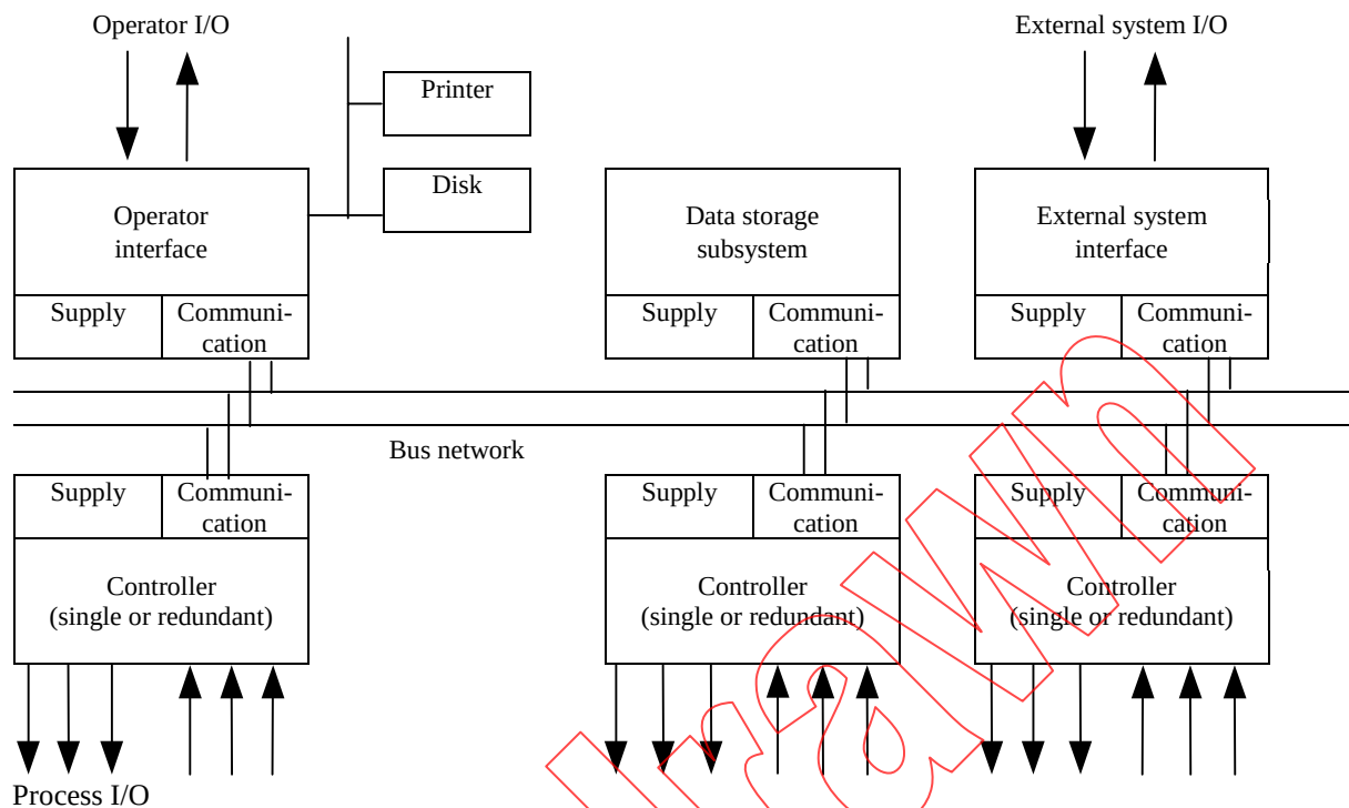
Figure C.2 – Generic physical system model
