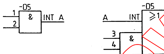
Figure 7 - Example of an interrupted internal connecting line
