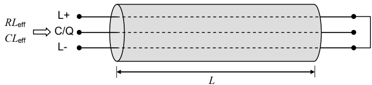
Figure 25 – Reference schematic for effective line capacitance and loop resistance
