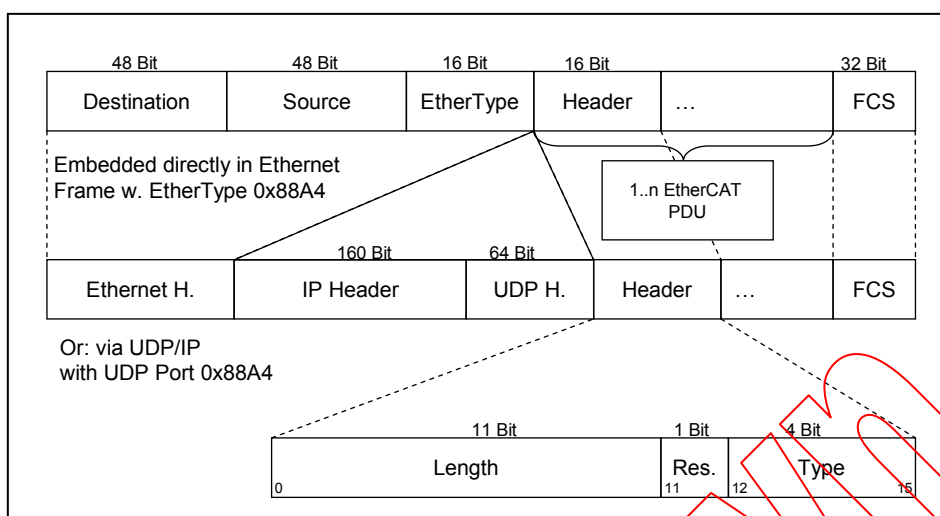
Figure 3 – Frame structure
