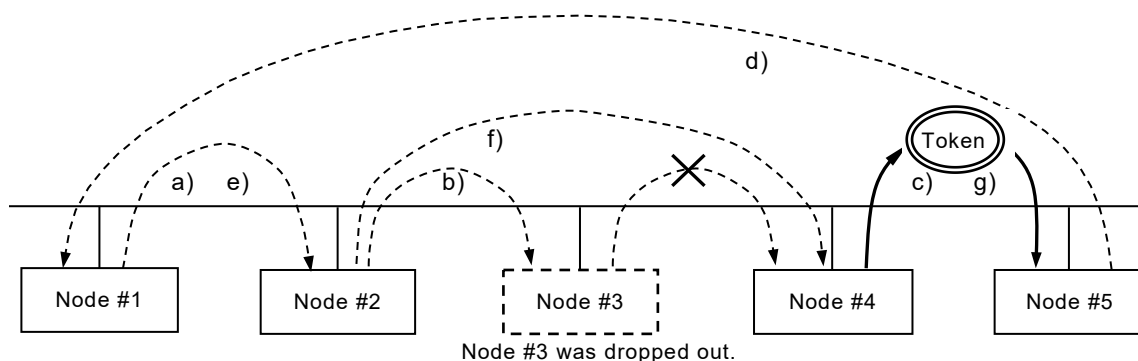
Figure 7 – Logical ring recovery
