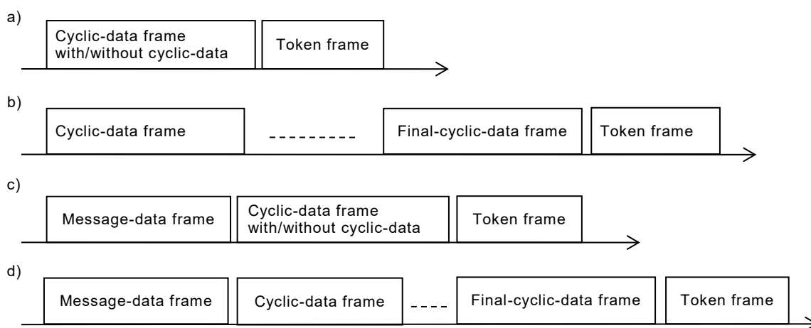
Figure 16 – Train of data frames and a token frame
