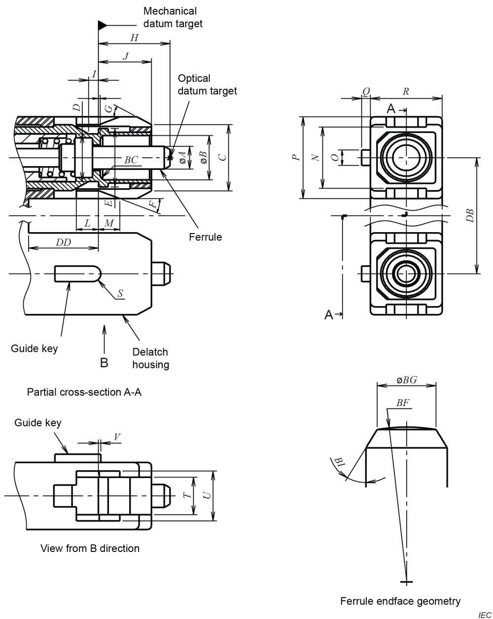
Figure 4 – Duplex PC plug connector interface
