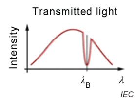
d) Transmitted spectral part of the incident light
