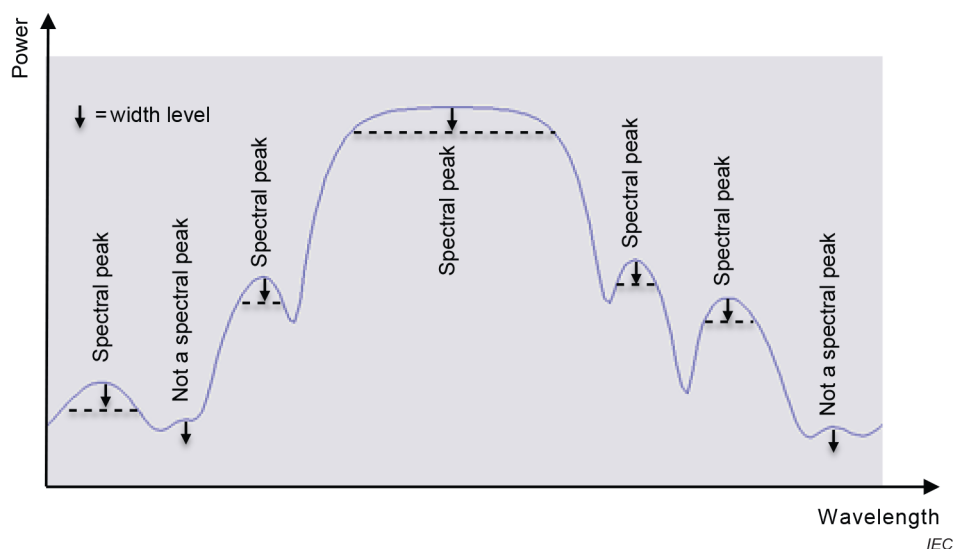
Figure A.3 – Spectral peaks in the case of serially multiplexed FBGs
