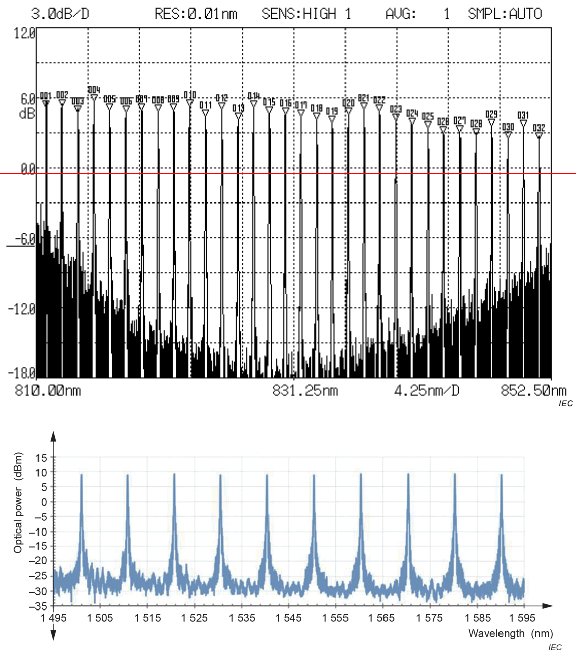
Figure 3 – Example of a reflection spectrum of a fibre Bragg grating array
