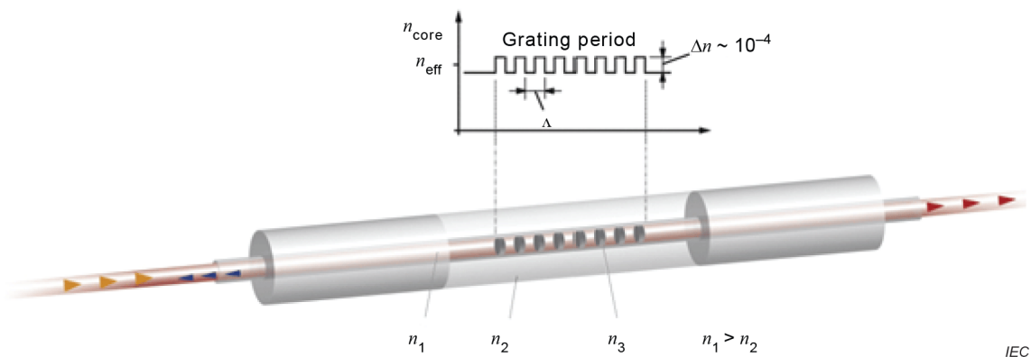
a) FBG refractive index profile and build-up
