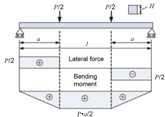
b) Load distribution
