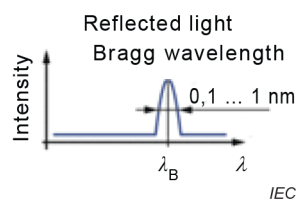
c) Reflected spectral part of the incident light
