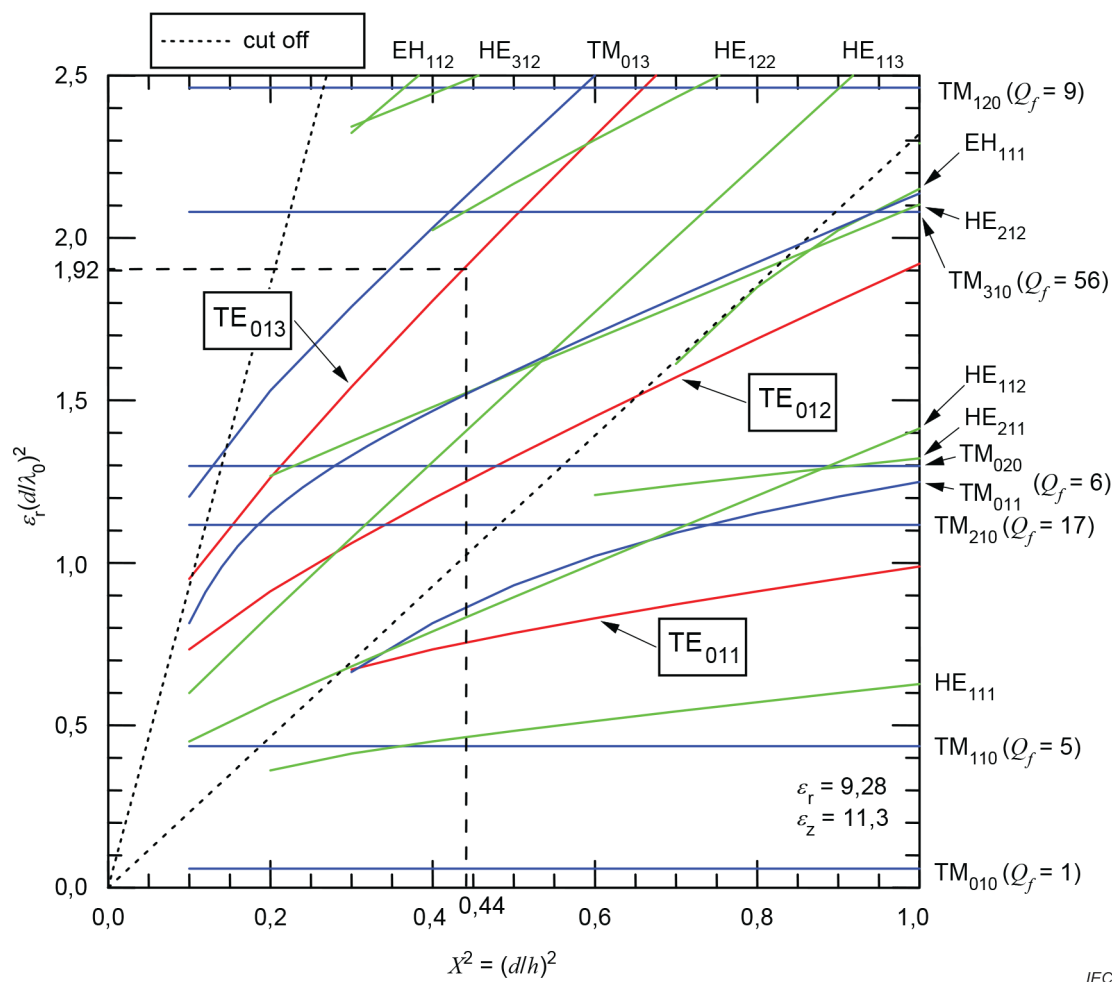
Figure A.7 – Mode chart to design TE 013 resonator short-circuited at both ends by parallel superconductor films [14] [28]
