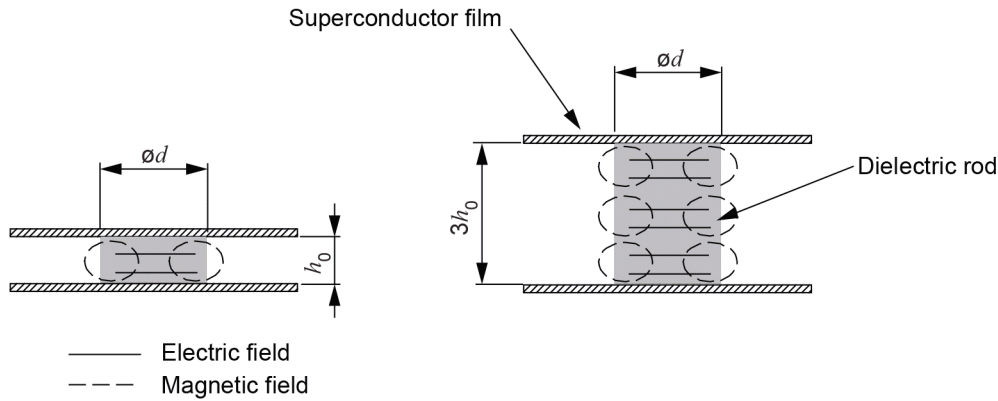
Figure A.4 – Configuration of standard dielectric rods for measurement of R_s and \tan \delta
