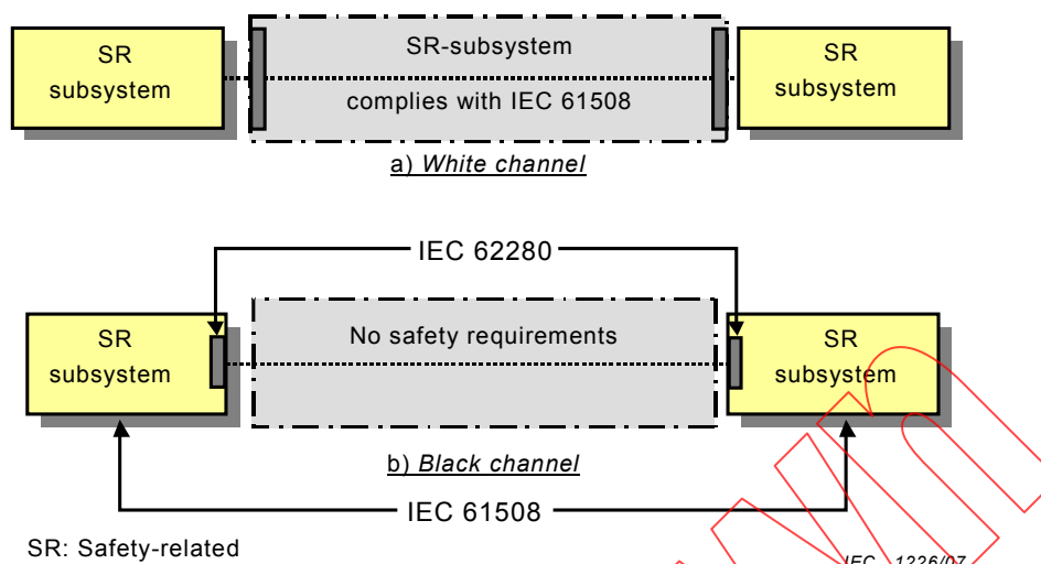
Figure 3 – Architectures for data communication: a) White channel; b) Black channel)
