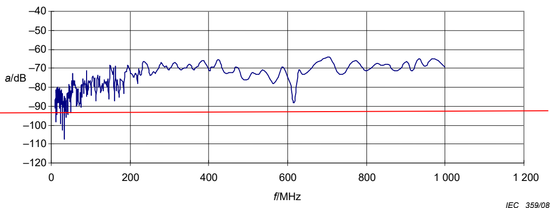
Figure 5 – Twinax 105 linear
