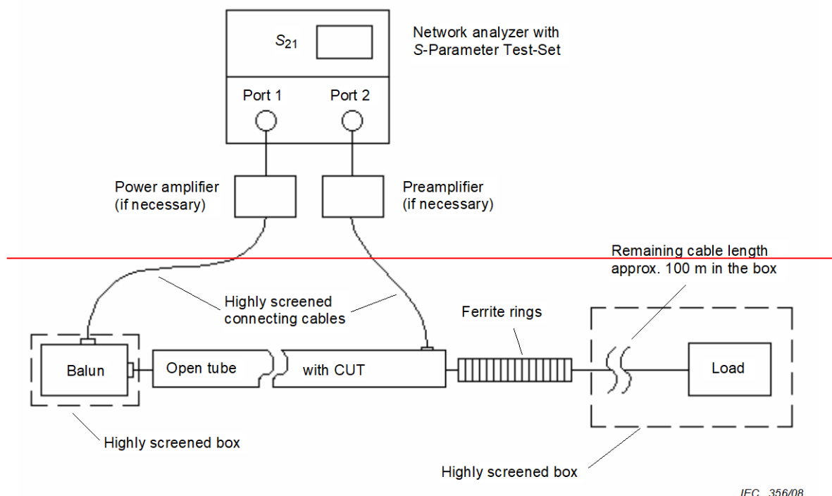
Figure 2 – Set-up to measure the coupling attenuation
