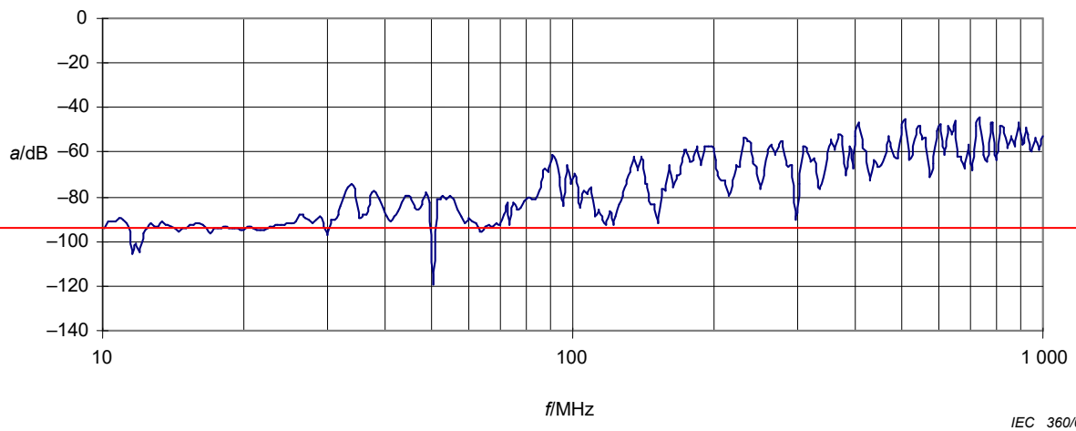
Figure 6 – FTP log
