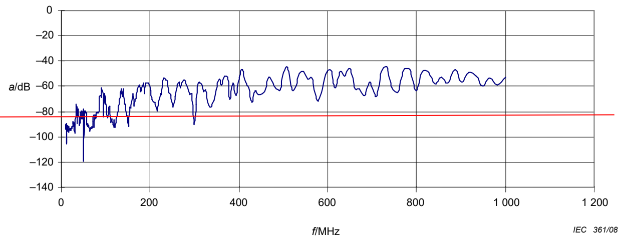
Figure 7 – FTP linear
