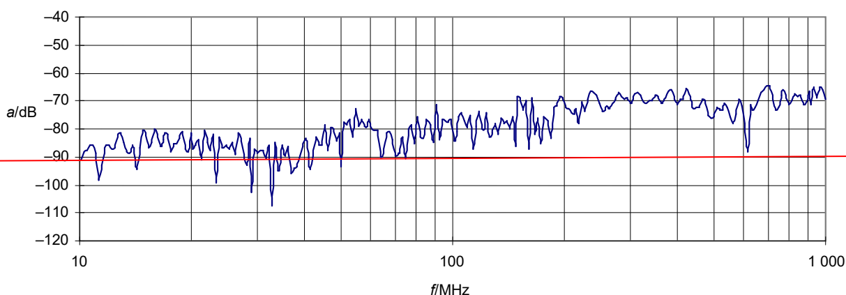
Figure 4 – Twinax 105 log
