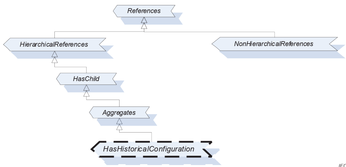
Figure 2 – ReferenceType hierarchy
