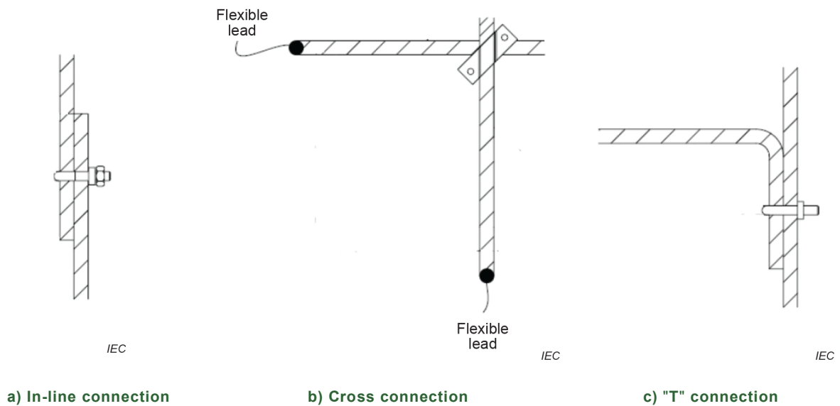
Figure 5 – Basic arrangement of specimen with clamped connection of reinforcing rods
