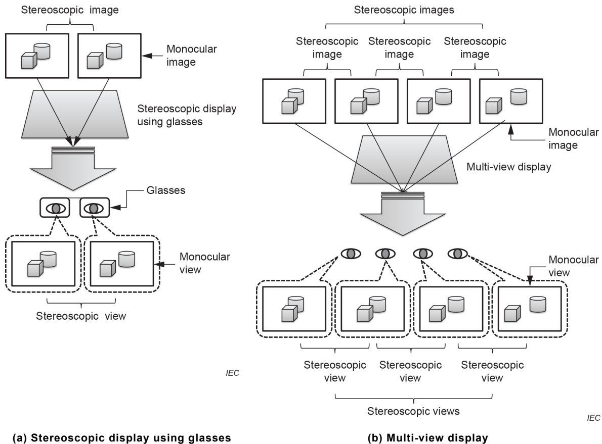
Figure A.3 – Stereoscopic images and stereoscopic views
