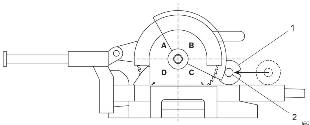
Figure 106 – Test probe
