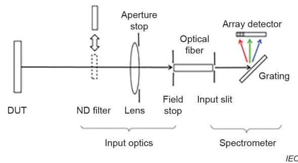
c) Spectroradiometer with spectrometer using grating and array detector
