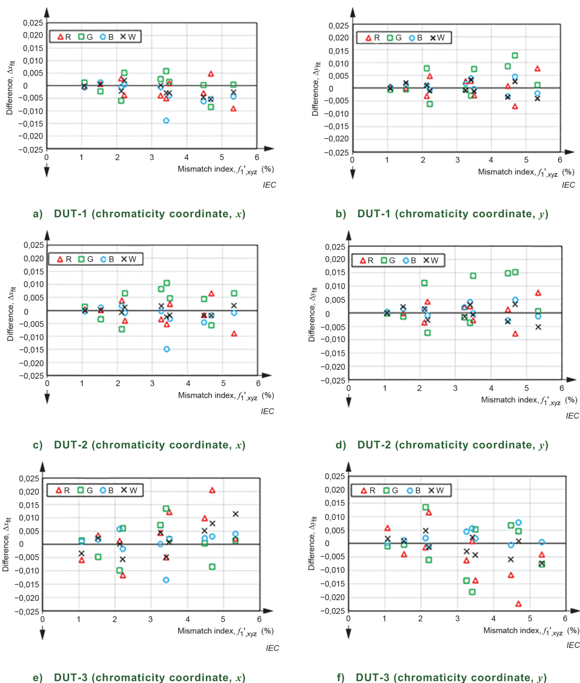
Figure 12 – Calculated chromaticity differences as a function of f_1', xyz
