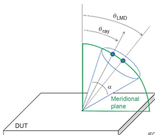
Figure 22 – Cone of light rays for calculating the tristimulus values measured by an LMD with the angular aperture, \alpha , and an optical axis at an inclination angle, \theta_{\text{LMD}}
