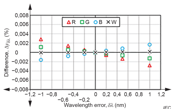
b) DUT-1 (chromaticity coordinate, y )
