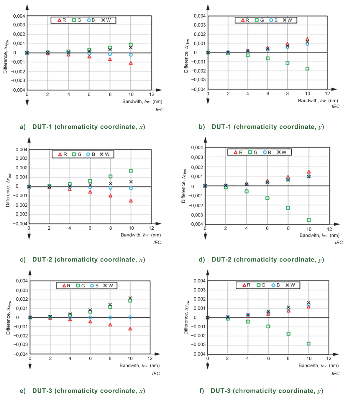
Figure 10 – Calculated chromaticity differences as a function of spectral bandwidth
