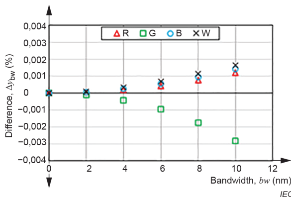
f) DUT-3 (chromaticity coordinate, y )
