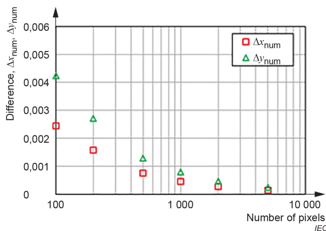
Figure 16 – Calculated chromaticity difference as a function of the number of pixels
