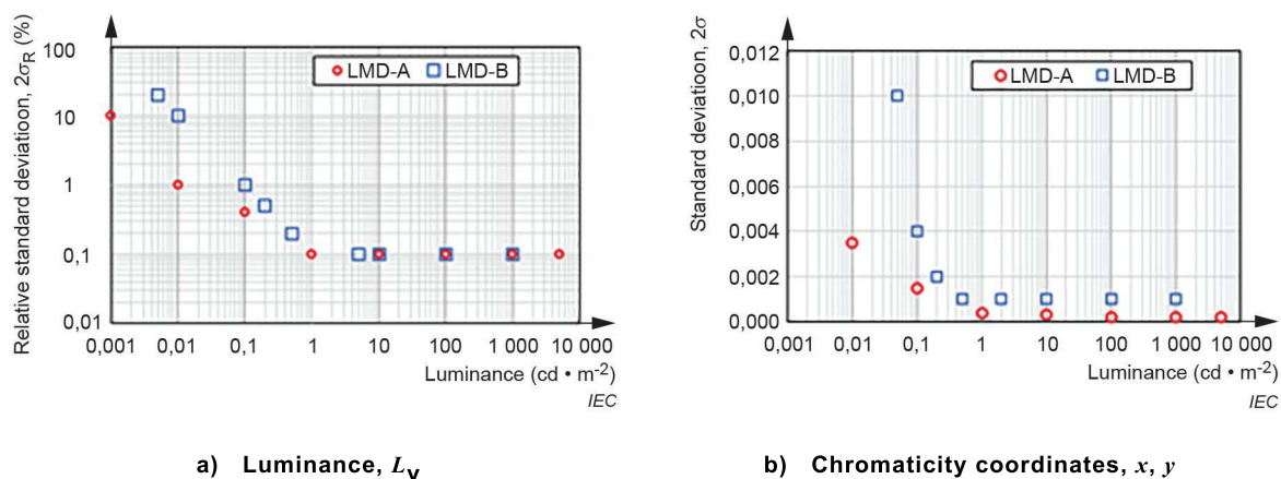
Figure 5 – Examples of the repeatability of an LMD as a function of luminance
