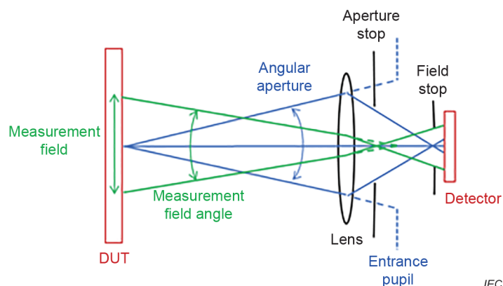
Figure 3 – Example of input optics for the luminance meters
