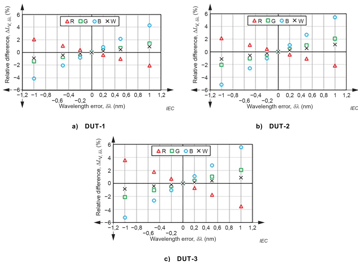
Figure 7 – Calculated relative luminance difference as a function of wavelength error
