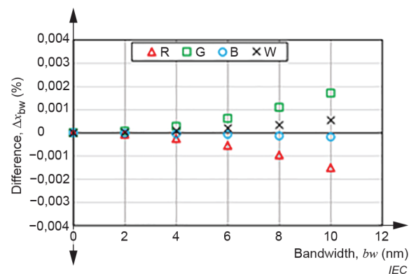
c) DUT-2 (chromaticity coordinate, x )
