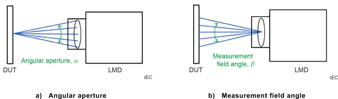
Figure 13 – Angular aperture and measurement field angle
