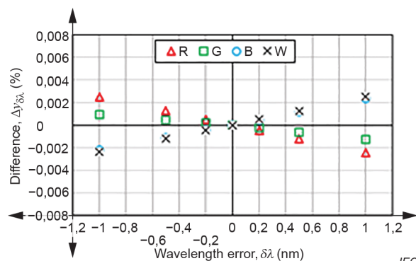
d) DUT-2 (chromaticity coordinate, y )
