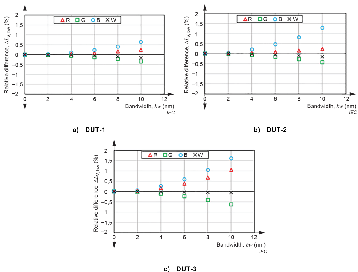
Figure 8 – Calculated relative luminance difference as a function of spectral bandwidth
