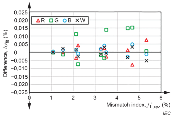
d) DUT-2 (chromaticity coordinate, y )
