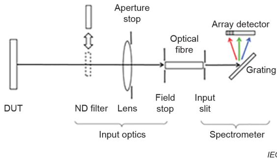
c) Spectroradiometer with spectrometer using grating and array detector
