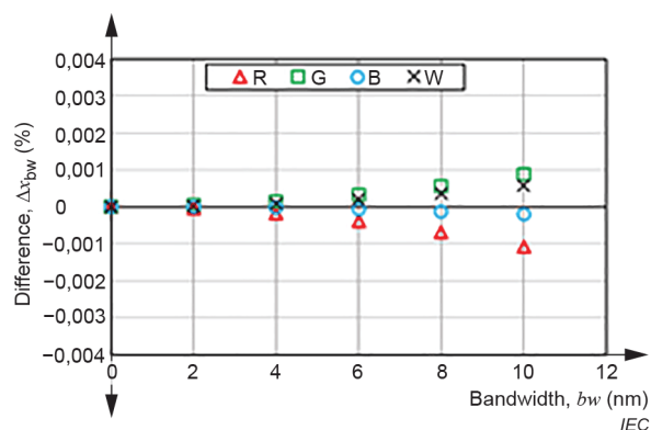
a) DUT-1 (chromaticity coordinate, x )
