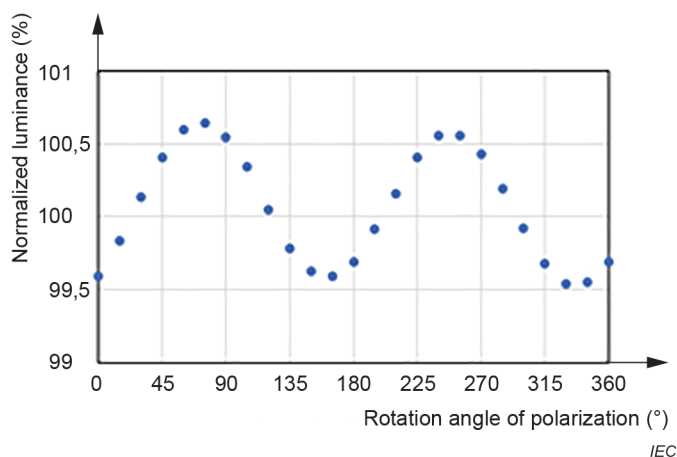
Figure 17 – Measured luminance variation as a function of the rotation angle of the polarizer
