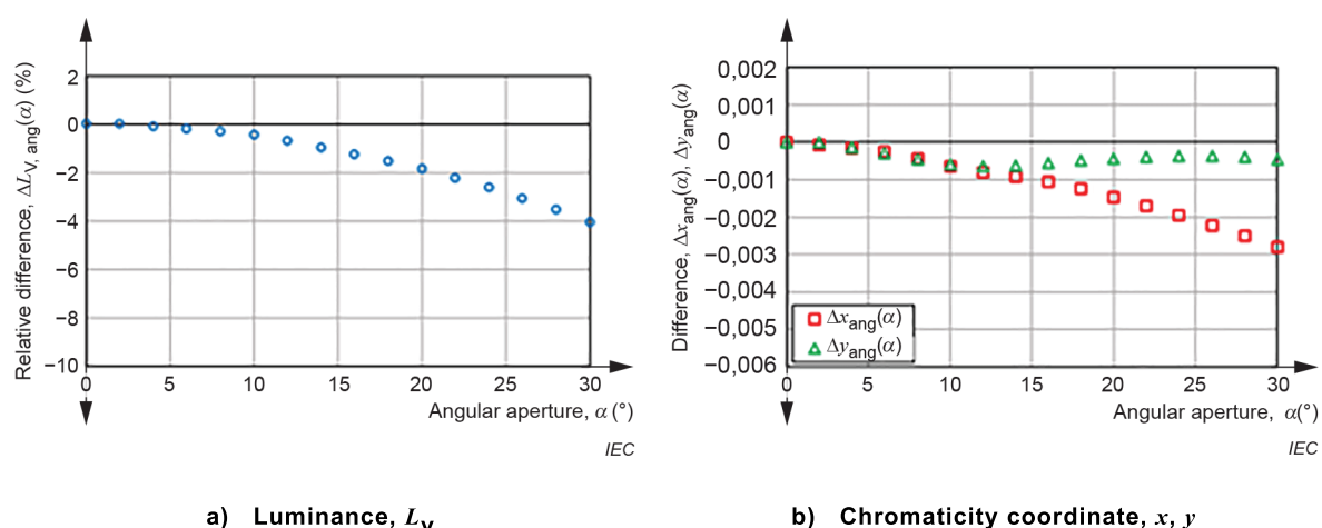
Figure 14 – Calculated relative luminance difference and chromaticity difference as a function of the angular aperture
