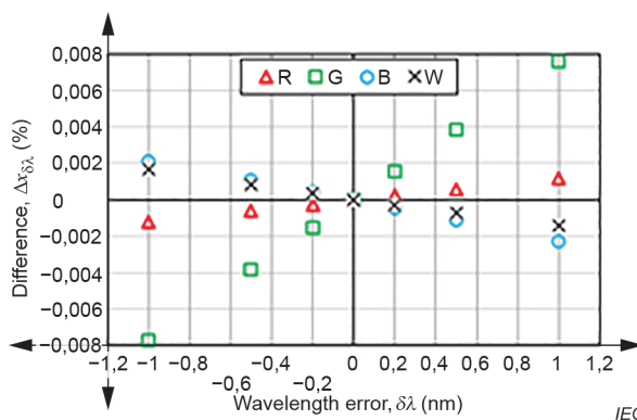
e) DUT-3 (chromaticity coordinate, x )
