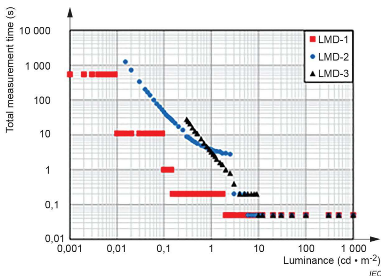
Figure 19 – Total measurement times for 0,3 % repeatability ( 2\sigma ) in three LMDs
