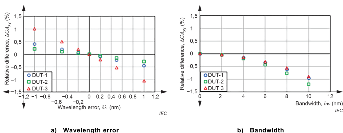
Figure 20 – Calculated relative difference, \Delta GA_{xy} , by spectroradiometers
