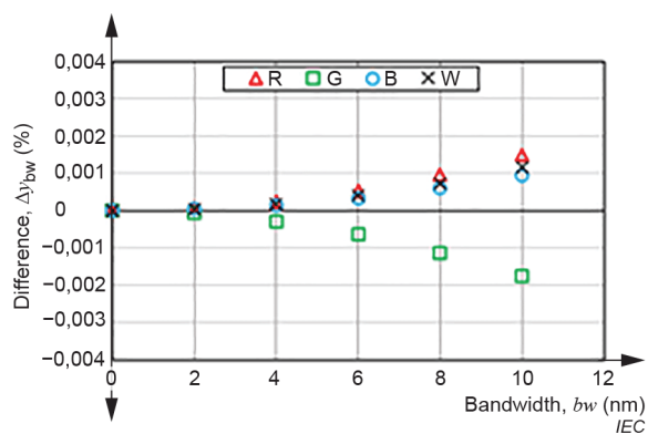
b) DUT-1 (chromaticity coordinate, y )
