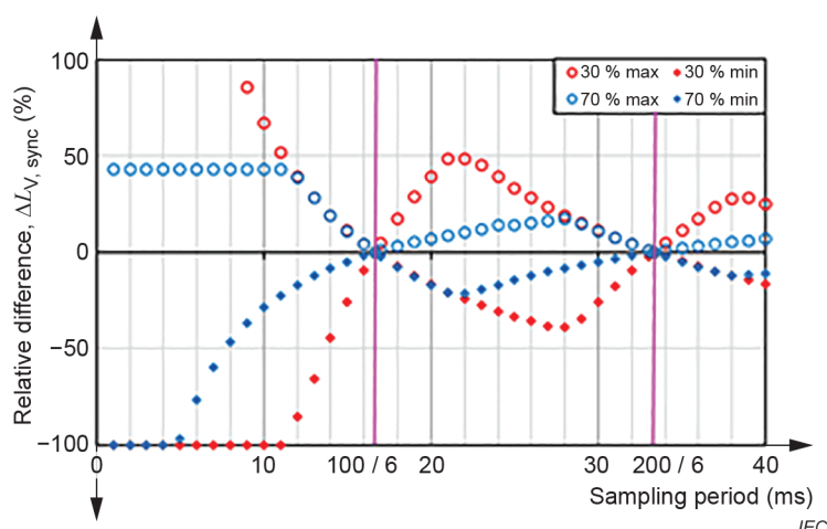
Figure 18 – Calculated relative luminance differences as a function of sampling period
