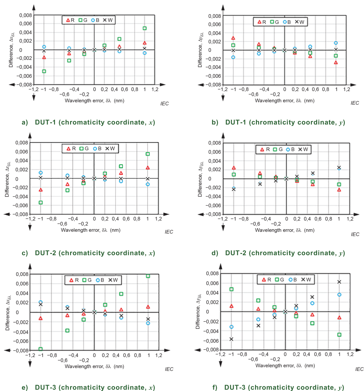
Figure 9 – Calculated chromaticity differences as a function of wavelength error
