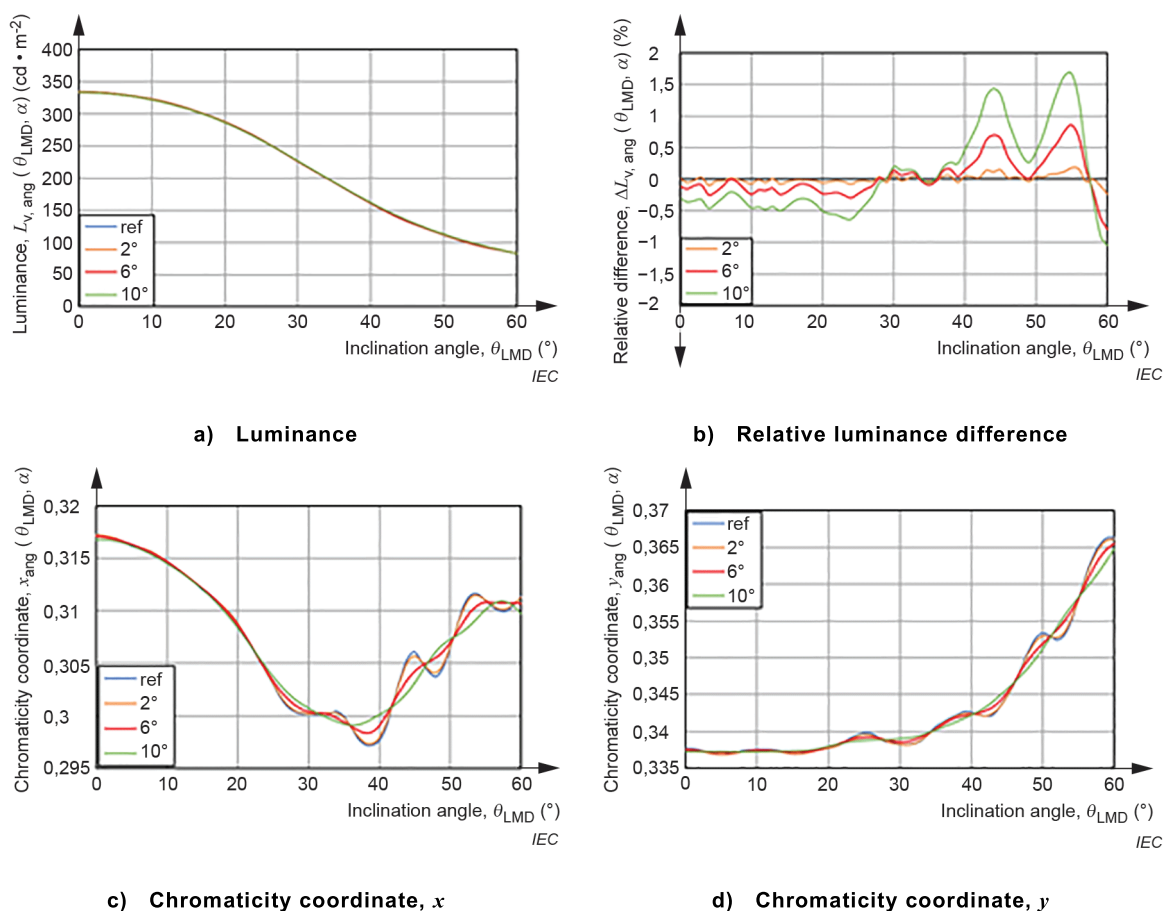
Figure 23 – Calculated luminance and chromaticity dependence as a function of the inclination angle for the 2°, 6°, and 10° angular apertures
