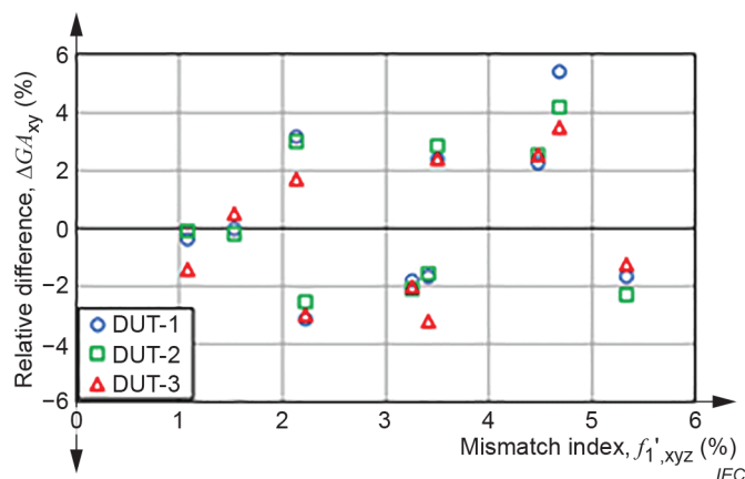
Figure 21 – Calculated relative difference, \Delta GA_{xy} , by colorimeters
