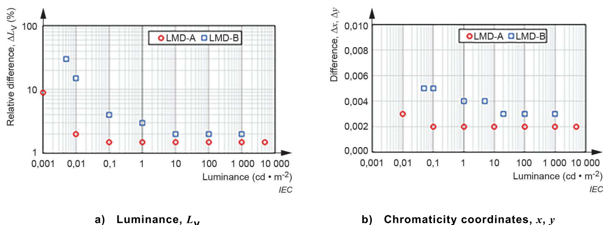
Figure 6 – Examples of the accuracy of an LMD as a function of luminance
