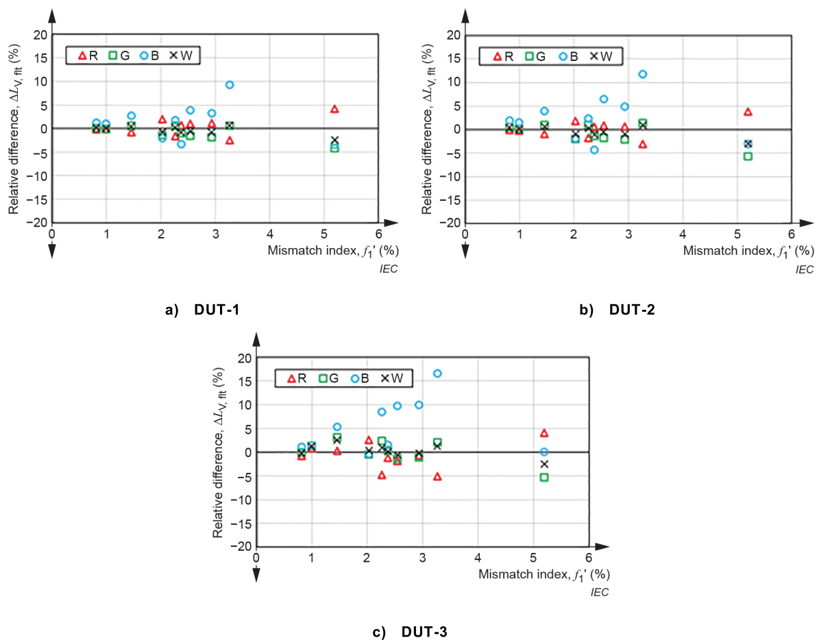
Figure 11 – Calculated relative luminance difference as a function of f_1'
