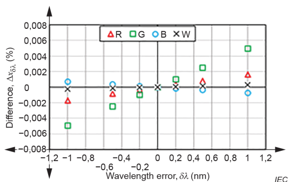
a) DUT-1 (chromaticity coordinate, x )
