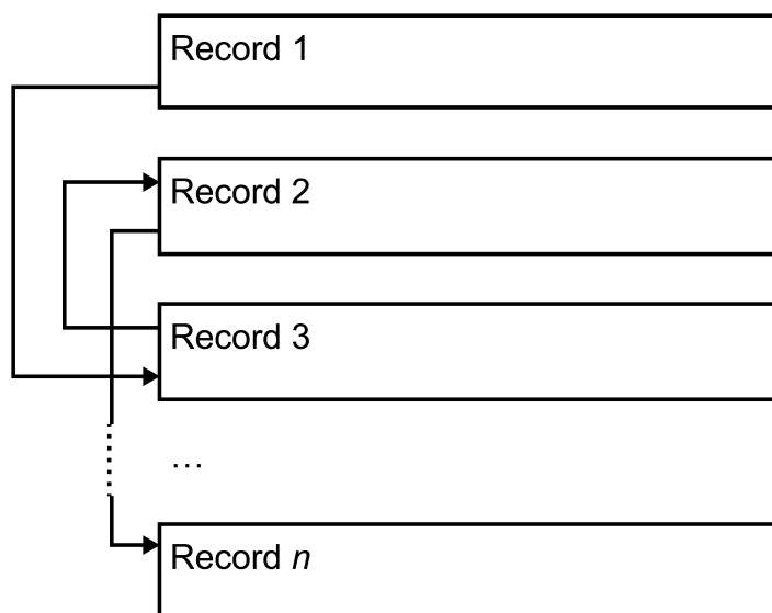
Figure 4—Reordering records
