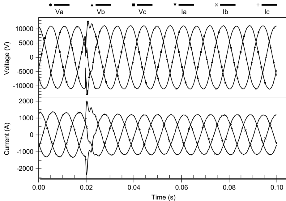
Figure 9—Low-frequency transient (capacitor switching)
