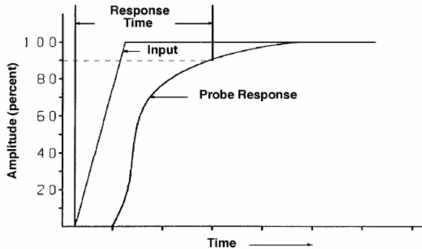
Figure 4—Typical response time curve
